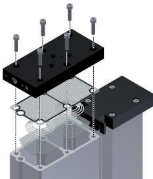
Retirer la plaque de soupapes antiretour
